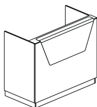
Riva_Bank140 140x70x105
