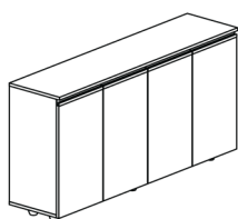
EXECUTIVE_STORAGE_WorkFullcover_CNSU160 160x39x78
