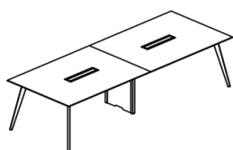
DESK_Sail_T240110 240x110x75
