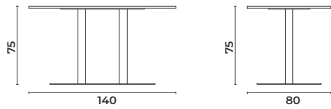
Pipe_Ct_E_14080H75
