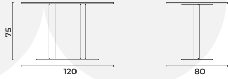
Pipe_Ct_12080H75
