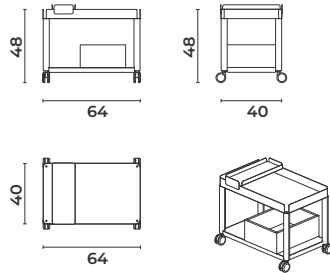
Cage_Trl_6440H48
