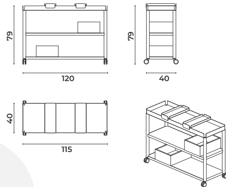
Cage_Trl_11540H79
